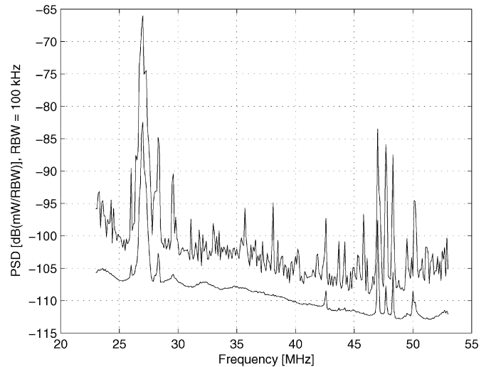
Fig. 9. Output of the analog receiver, summarizing 2 days of continuous observations, with transfer functions of the analog receiver, coaxial cable, active balun, and antenna (IME) removed. Top : Maximum value ever observed, Bottom : Mean.
