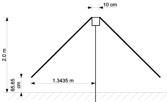
Fig. 3. Key dimensions of the dipole.
