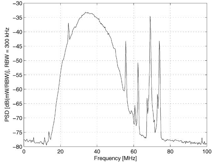
Fig. 8. Output of the analog receiver: Integrated (i.e., mean) power spectral density after 2 days of continuous measurement. No attempt has been made to calibrate the frequency response. Strong signals above 50 MHz are analog TV stations. The noise floor at about -78 dB is due to the spectrum analyzer.
