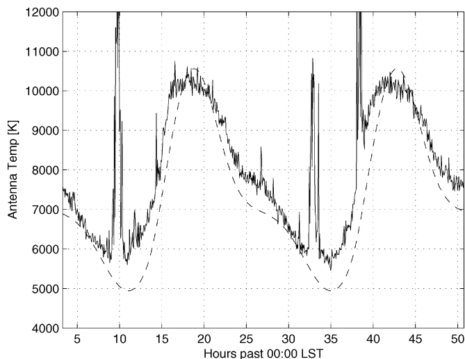
Fig. 11. 39.0 MHz result from Fig. 10 (solid) shown with result predicted by extrapolation from 408 MHz sky survey (dashed).
